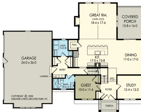
FIRST FLOOR PLAN Scale: 1/4" = 1'-0" Living Area = 1443 Sq. Ft. 9'-0" Ceiling Height
