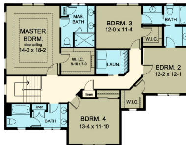
SECOND FLOOR PLAN Scale: 1/4" = 1'-0" Living Area = 1540 Sq. Ft.
