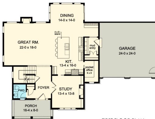
FIRST FLOOR PLAN Living Area = 1430 Sq. Ft. 9'-0" Ceiling Height
