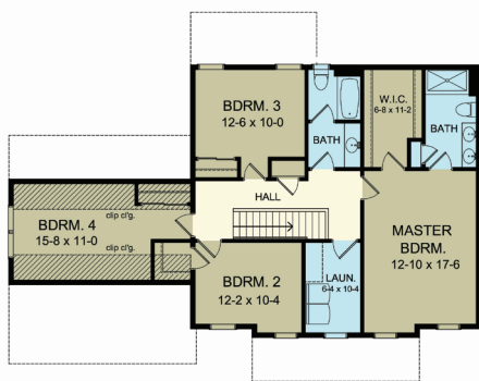
SECOND FLOOR PLAN Living Area = 1257 Sq. Ft.
