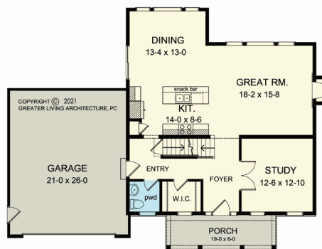
FIRST FLOOR PLAN Living Area = 1076 Sq. Ft. 7'-0" Ceiling Height
