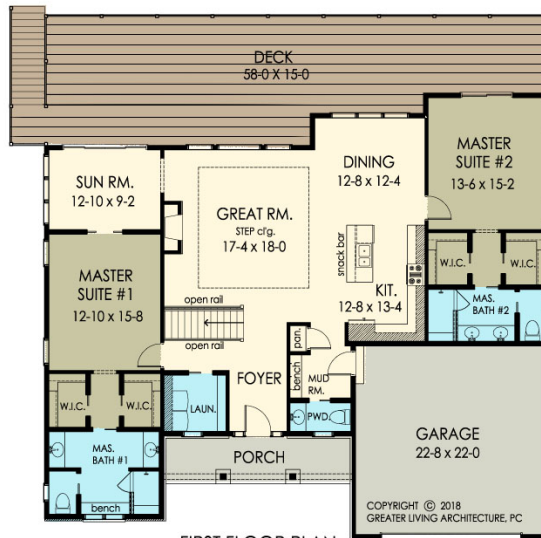
FIRST FLOOR PLAN Scale: 1/4" = 1'-0" Living Area = 1967 Sq. Ft. 42'-0" Wide 9'-0" Ceiling Height 60'-0" Deep
