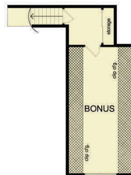
BONUS RM. FLOOR PLAN SCALE: 1/4" = 1'-0" Living Area = 475 Sq. Ft.
